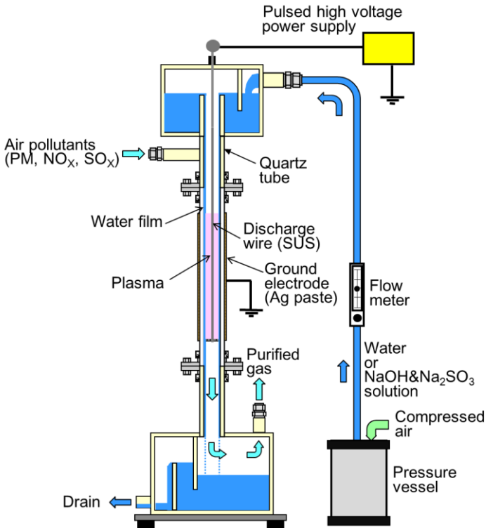
Fig. 1. Schematics of wet-type plasma reactor
