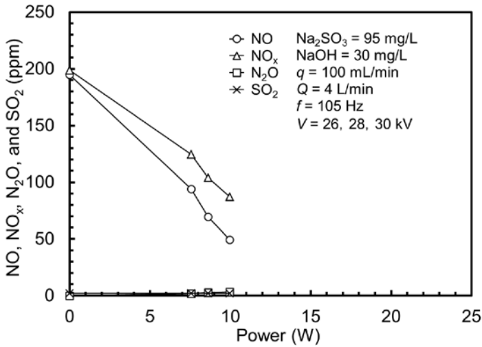
Fig. 9. Simultaneous removal of \text{NO}_x and \text{SO}_x under coexisting with nanoparticle for the pulse frequency of 105 Hz (total flow rate = 4 L/min, the ground electrode length = 260 mm).
