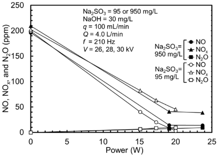
Fig. 10. Effect of \text{Na}_2\text{SO}_3 concentration on \text{NO}_x removal for the pulse frequency of 210 Hz (total flow rate = 4 L/min, the ground electrode length = 260 mm).
