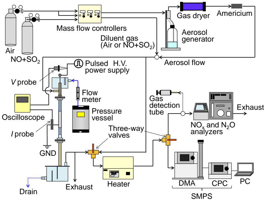
Fig. 2. Experimental setup for simultaneous removal of nanoparticle, \text{NO}_x , and \text{SO}_2
