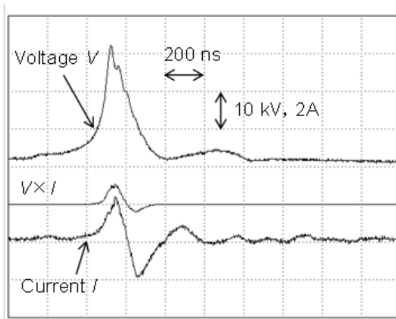
Fig. 3. Voltage, current, and instantaneous power waveforms.
